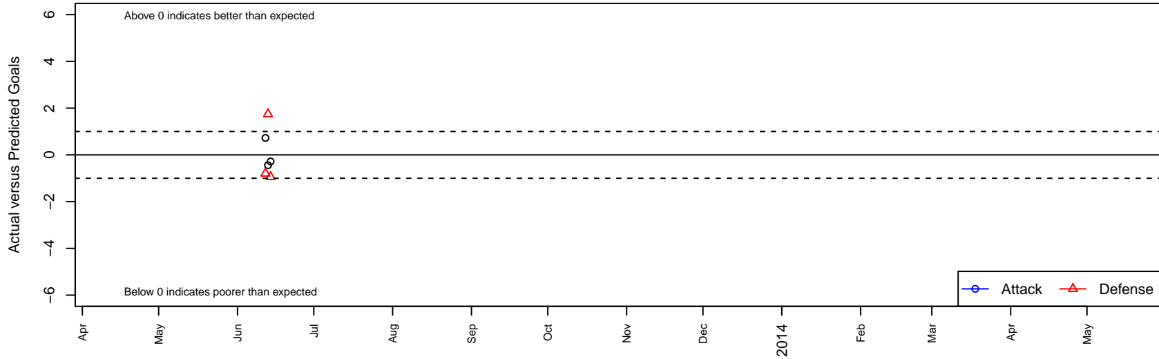
Eclipse Phoenix 99 B98 Dots are actual minus expected GF (blue circles) and GA (red triangles). Blue line is smoothed change in attack strength. Red is smoothed change in defense strength.
